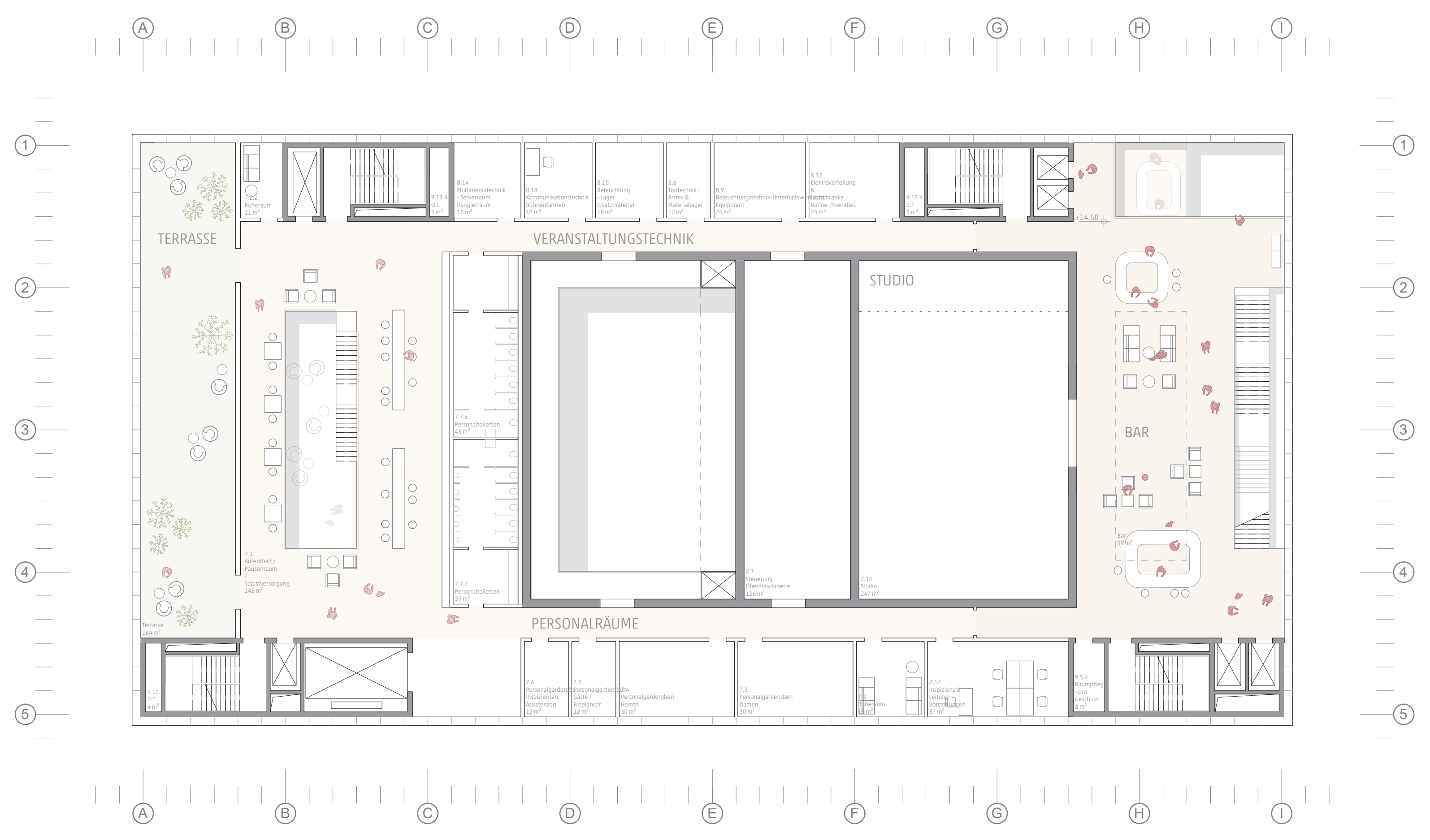
Grundriss 4.0G | 1:200
